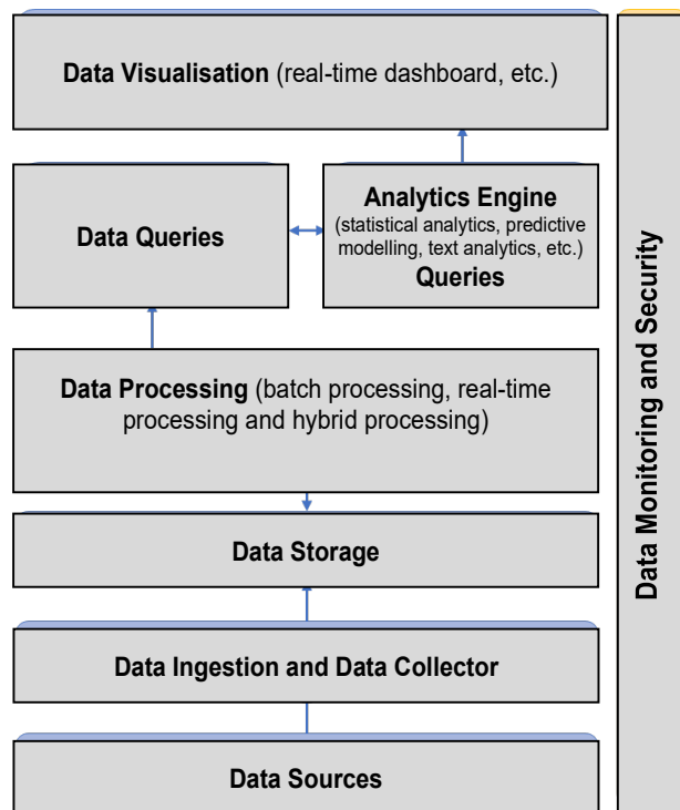
Figure 1. Stages in big data processing
